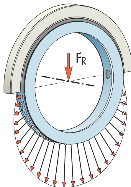
RADIAL LOADS
