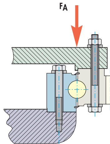
SUPPORTED LOAD
