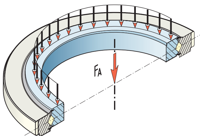
AXIAL LOADS
