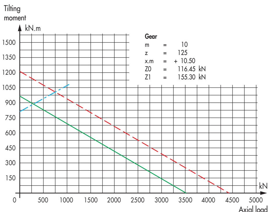
CURVES OF BEARING 06 1116 00
