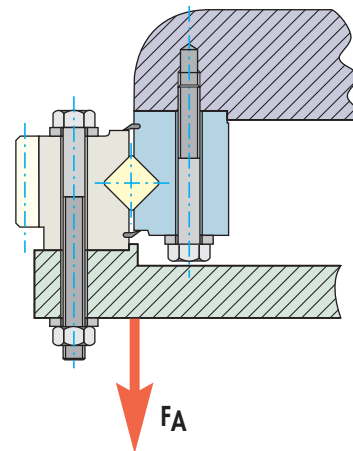
HANGING LOAD
